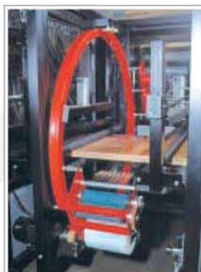
The prestretching device for increasing the wrapping quality, lowering the packaging price and foil consumption by 20 - 30 %. This secures a fast rate of return of investment.
